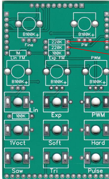
Pots 'n' sockets PCB
