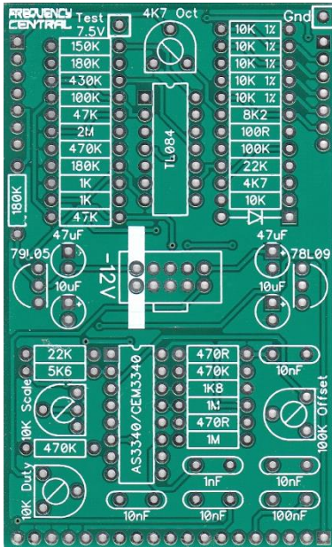
Main PCB
